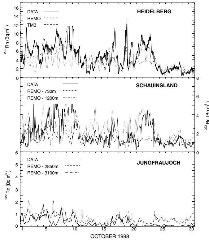
Fig. 7. Same as Fig. 5, but for October 1998.
