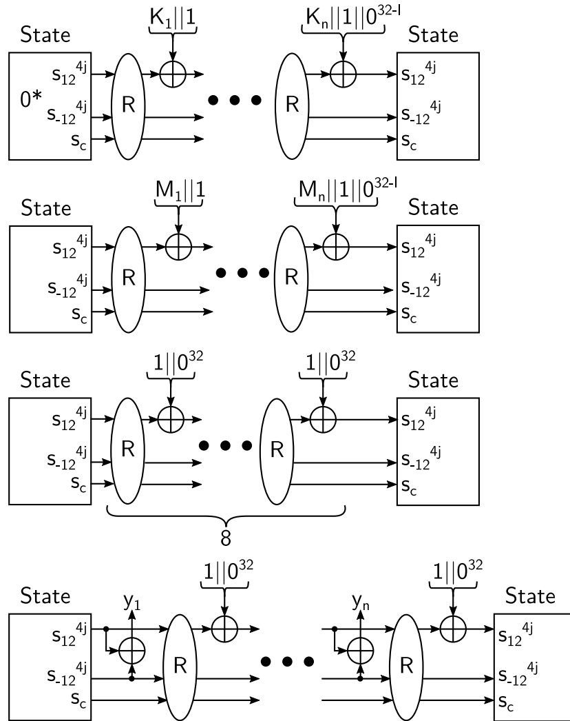
Figure 12: Subterranean deck.
