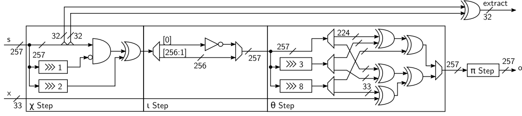
Figure 3: Subterranean duplex combinatorial circuit.
