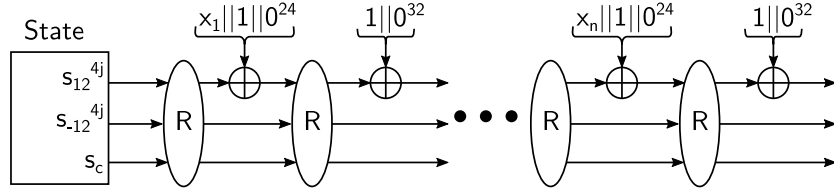
Figure 5: Subterranean absorb with operation unkeyed.
