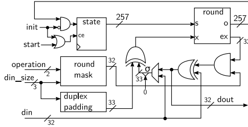
Figure 4: Subterranean single-round duplex logic.
