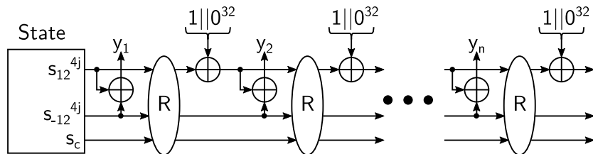
Figure 9: Subterranean squeeze.
