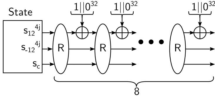
Figure 10: Subterranean blank.
