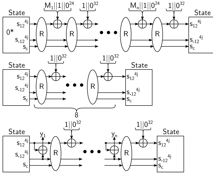
Figure 11: Subterranean XOF.
