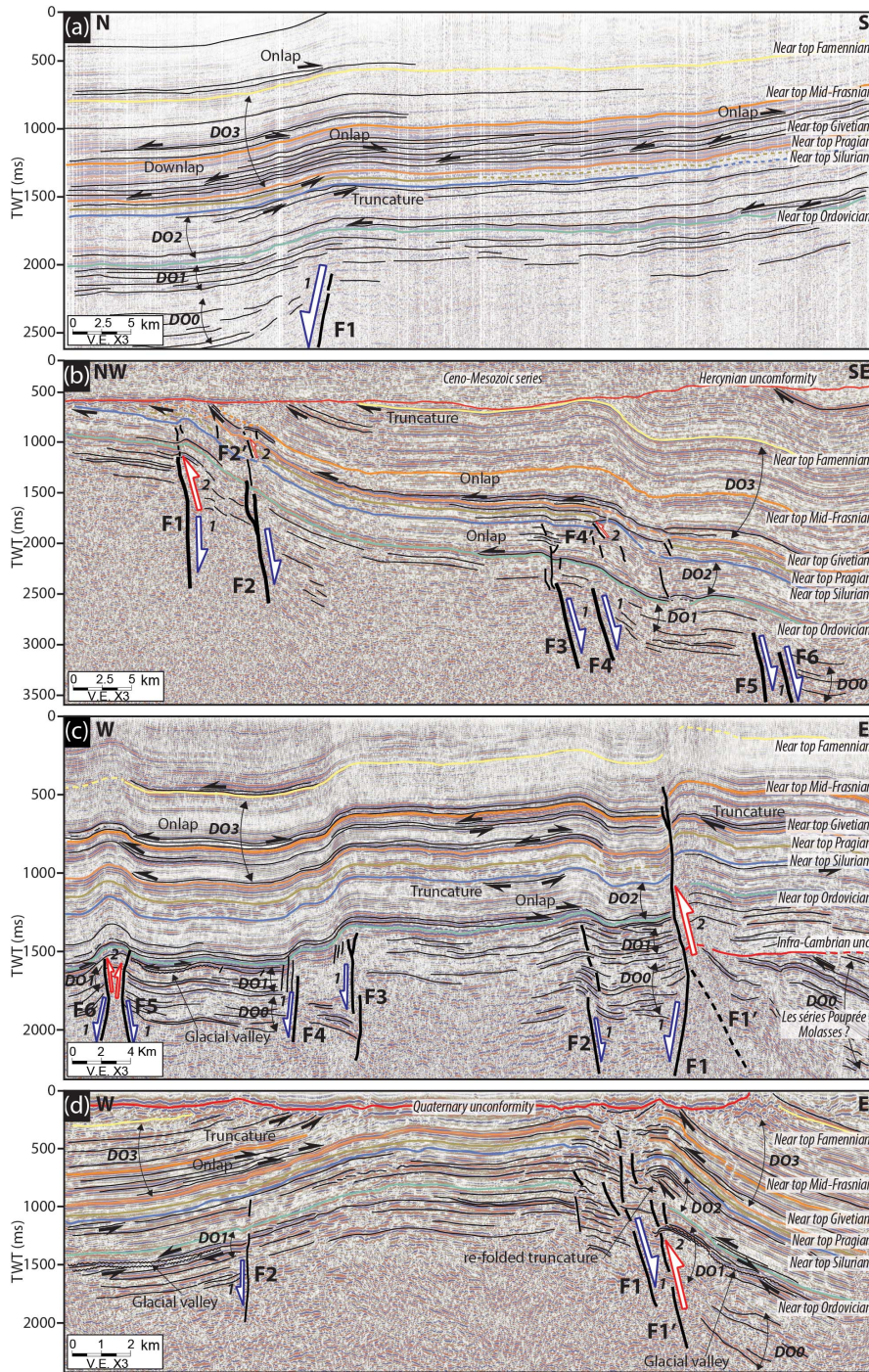
Figure 7. (a) N–S interpreted seismic profile in the Ahnet Basin near Erg Teguentour (near Arak-Foum Belrem Arch, westward interbasin boundary secondary arch) showing steeply dipping northward basement normal blind faults associated with forced folding. (b) NW–SE interpreted seismic profile of near Azzel Matti Arch (interbasin principal arch) showing steeply dipping southeastward basement normal blind faults associated with forced folds. The westernmost structures are featured by reverse fault related propagation fold. (c) W–E interpreted profile of the Ahnet Basin (Arak-Foum Belrem Arch, westward interbasin boundary secondary arch) showing horst and graben structures influencing Paleozoic tectonics associated with forced folds. (d) W–E interpreted seismic profile of Bahar el Hammar in the Ahnet Basin (Ahnet intra-basin secondary arch) showing steeply dipping normal faults F1 and F2 forming a positively inverted horst associated with folding. Multiple activation and inversion of normal faults are correlated with divergent onlaps (wedge-shaped units): DO0 infra-Cambrian extension, DO1 Cambrian–Ordovician extension, DO2 Silurian extension with local Silurian–Devonian positive inversion, and DO3 Frasnian–Famennian extension–local compression. See Fig. 2 for map and cross-section location.
