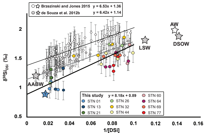
Figure 3. \delta^{30}\text{Si}_{\text{DSi}} versus the inverse of DSi concentration for this study (coloured circles identified by station; STN), de Souza et al. (2012b; grey circles) and Brzezinski and Jones (2015; open circles) for waters > 1000 m depth. Equations reported in the figure refer to linear regressions produced for each dataset (de Souza et al., 2012b – grey line, y = 6.42x + 1.14 ; Brzezinski and Jones, 2015 – thin black line, y = 6.53x + 1.36 ; this study – thick black line, y = 8.18x + 0.89 ). The statistics associated with each linear regression are as follows: de Souza et al. (2012b) – standard deviation of the slope ( \text{SD}_s ) = 0.31, standard deviation of the y ( \text{SD}_y ) = 0.06, standard deviation of the intercept ( \text{SD}_i ) = 0.02, R^2 = 0.86 , n = 58 ; Brzezinski and Jones (2015) – \text{SD}_s = 0.32 , \text{SD}_y = 0.07 , \text{SD}_i = 0.02 , R^2 = 0.83 , n = 83 ; these results – \text{SD}_s = 1.1 , \text{SD}_y = 0.17 , \text{SD}_i = 0.08 , R^2 = 0.64 , n = 29 . The stars presented in this figure represent the end-members for the AABW, LSW, and DSOW previously published by de Souza et al. (2012b – grey stars), the Arctic Water (AW) previously published by Brzezinski and Jones (2015 – the white star), and an unknown end-member (blue star, see text for details).
