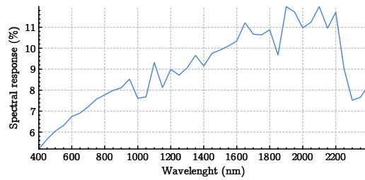
Fig. 10. Asphalt pavement, spectral response and angular distribution.
