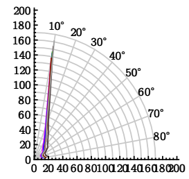
Fig. 8. The work zone signaling cone (grey reflective strip), spectral response and angular distribution.
