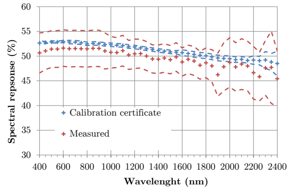
a. Spectral response at 10°.
