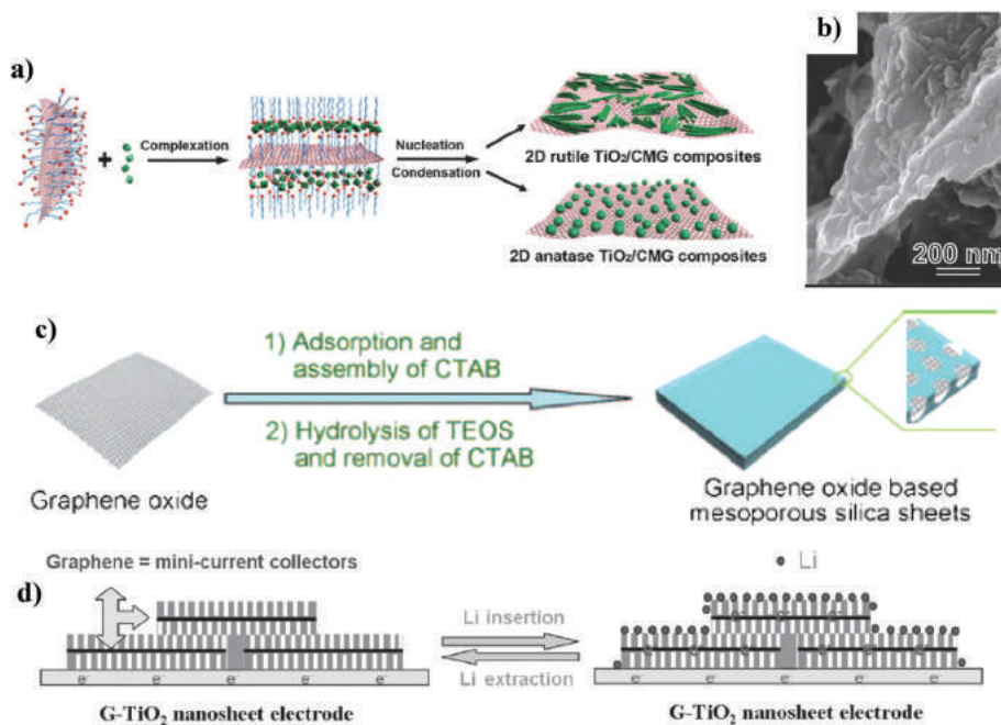
Fig. 109 Examples of 2d nanocomposites based on GRMs. (a) Assembly steps for a TiO 2 /GO nanocomposite from SDS-modified graphene sheets. (b) SEM image of a rutile TiO 2 /GO nanocomposite. (c) Fabrication process for GO based mesoporous silica sheets through the hydrolysis of tetraethylorthosilicate (TEOS), with cationic surfactant cetyl trimethylammonium bromide (CTAB)-functionalized GO as the template. (d) Lithium insertion and extraction in GMR sheets, where graphene acts as mini-current collectors during discharge and charge processes, facilitating the rapid diffusion of electrons during cycling processes. 2144
