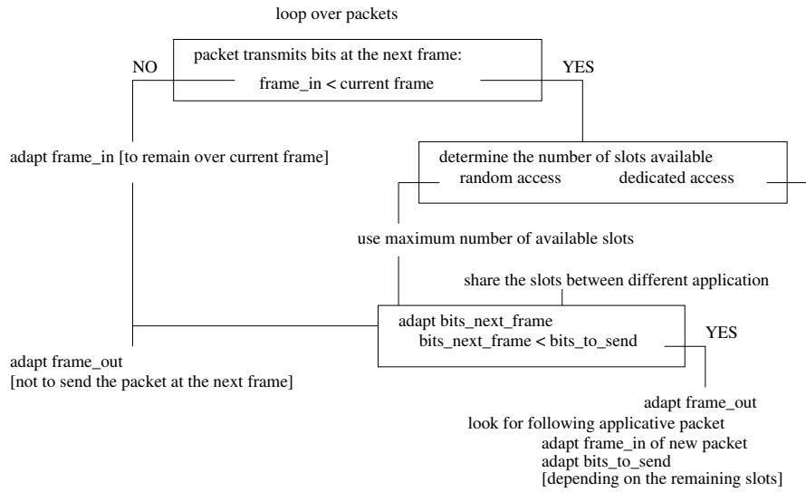
Fig. 4. adaptBitNextFrame() method flowchart
