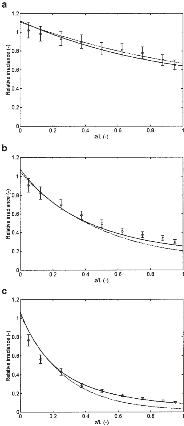
Figure 7. (a–c) Comparison between attenuation profiles in the photobioreactor and experimental irradiances measured with a spherical quantum sensor of 3 mm diameter (solid line: \frac{G_{\Sigma}}{q_0} , dotted line: \frac{G}{q_0} , \circ : experimental values). (a) C_X = 0.09 g/L or \tau = 4 , (b) C_X = 0.25 g/L or \tau = 10 (c) C_X = 0.49 g/L or \tau = 20 ).
