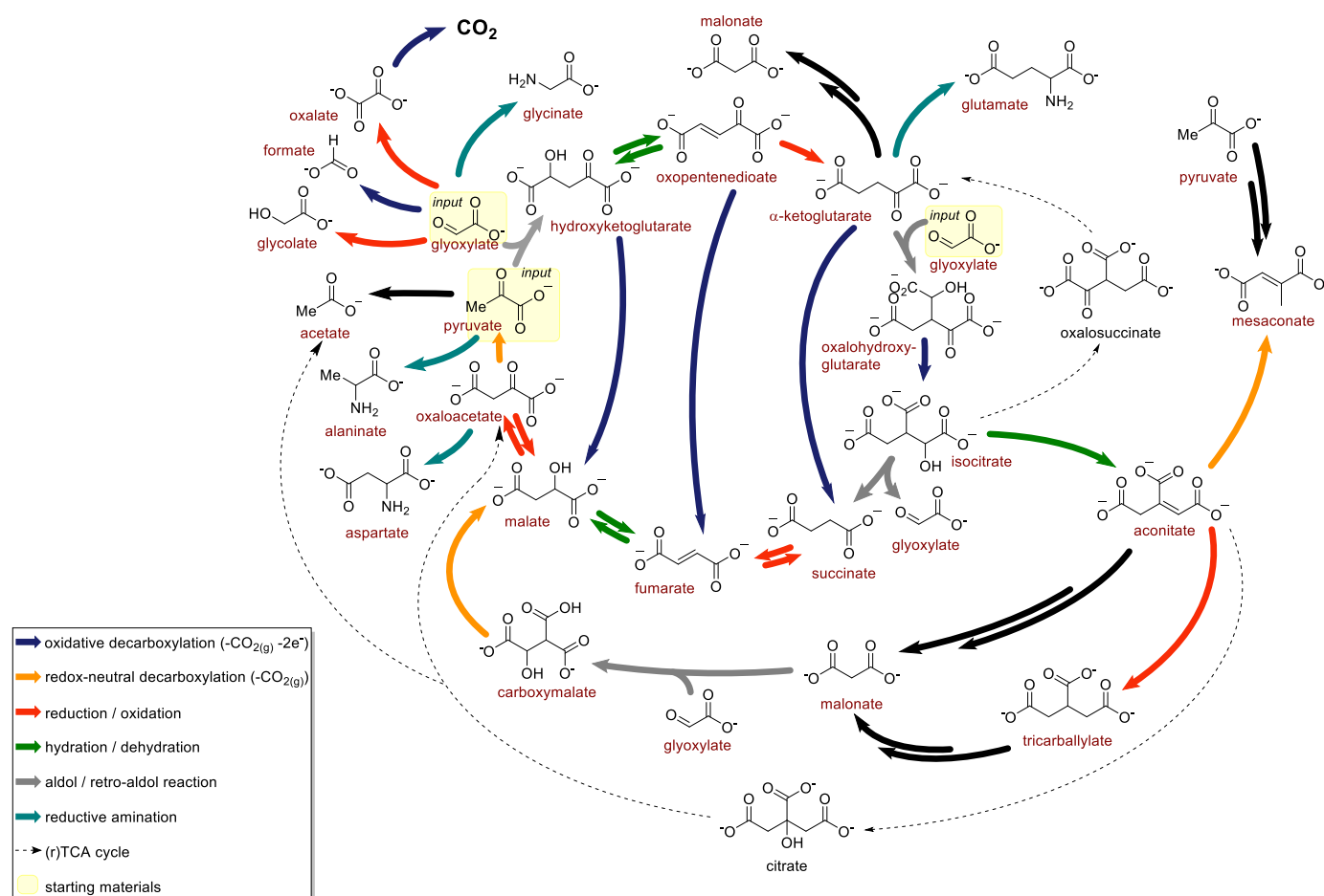
Figure 4. Reaction network arising from pyruvate and glyoxylate, promoted by \text{Fe}^{2+} in water at 70\text{ }^\circ\text{C} . (r)TCA cycle reactions not detected within the network are shown as dotted arrows.
