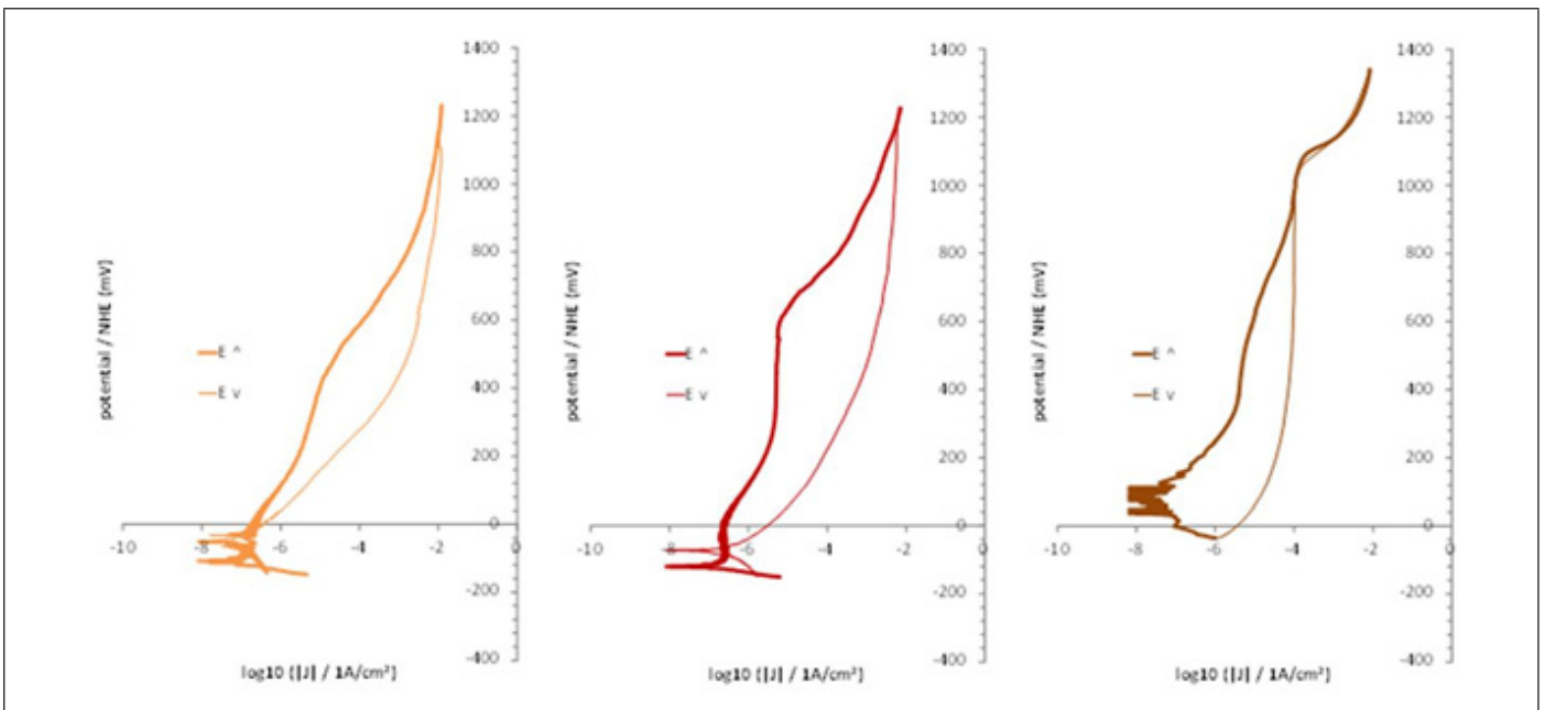
Figure 7: E-J curves obtained during the cyclic polarization of the two of the three Cr-richest alloys (left: Co-20Cr, middle: Co-25Cr, right: Co-30Cr).
