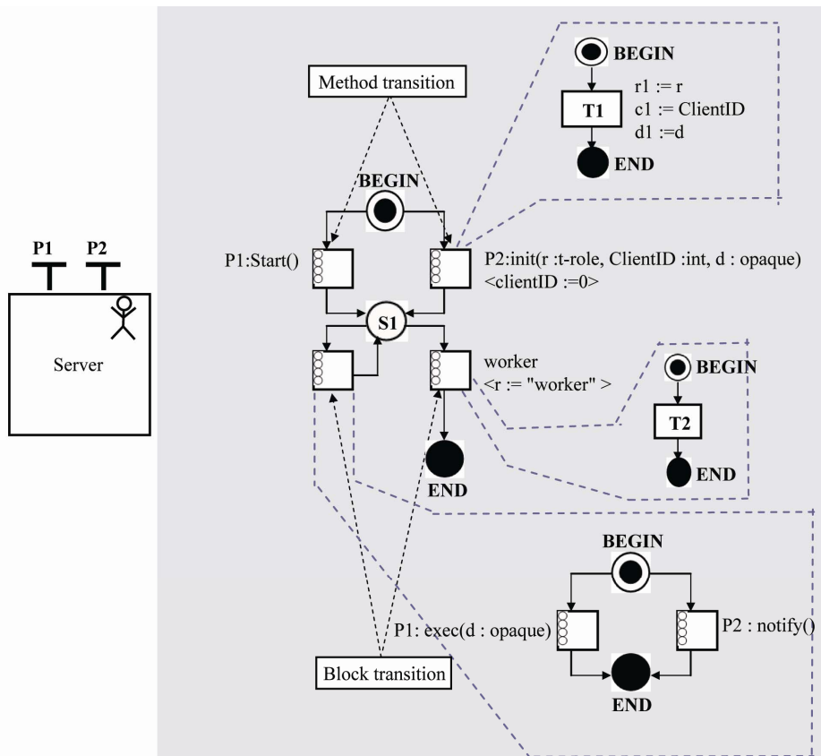
Figure 7. Client-Server LfP-BD (CS-LfP-BD).
