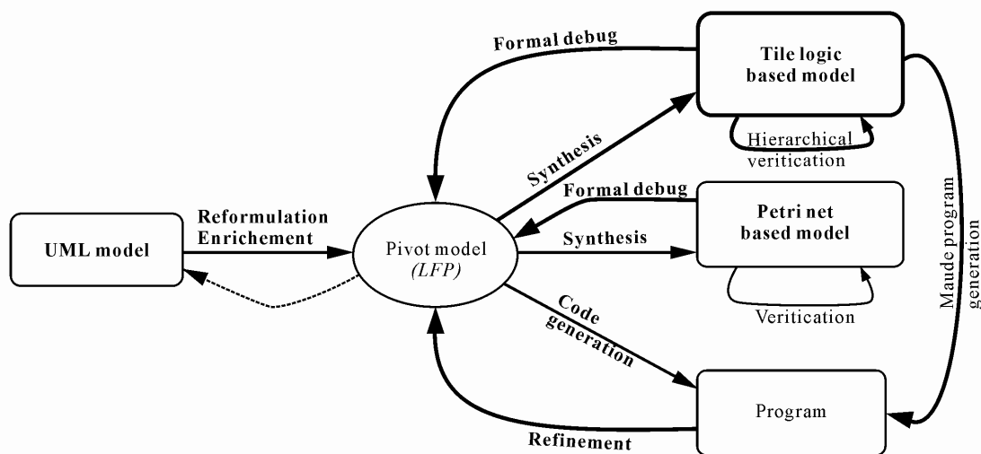
Figure 3. LfP methodology extension.
