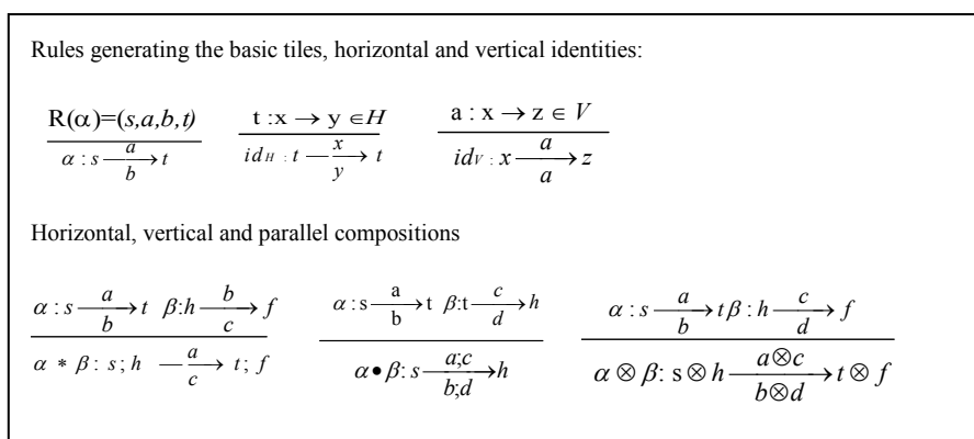
Figure 2. Inference rules.
