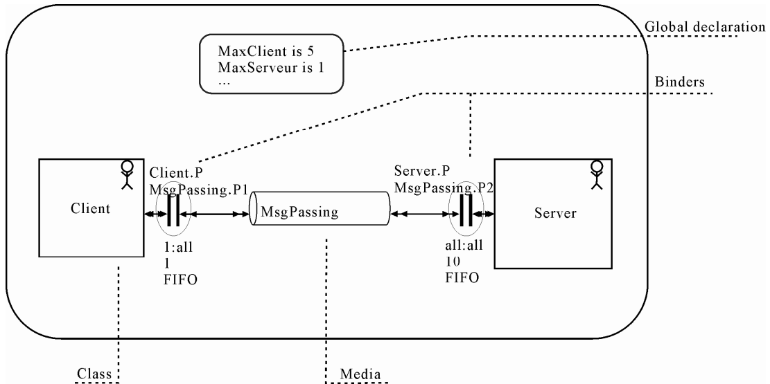
Figure 6. Client-Server LfP-AD (CS-LfP-AD).
