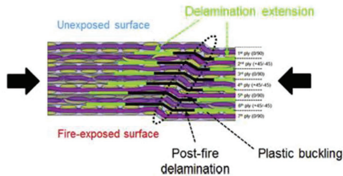
Figure 29. Damage mechanisms in woven-ply quasi-isotropic C/PPS laminates subjected to compression after fire exposure: a) local microbuckling of fiber bundles at the crimp in a 5-harness satin weave. b) Delamination and global plastic buckling induced by postfire delamination and the formation of plastic kink bands. Adapted with permission. [234] Copyright 2017, Elsevier Science Ltd.
