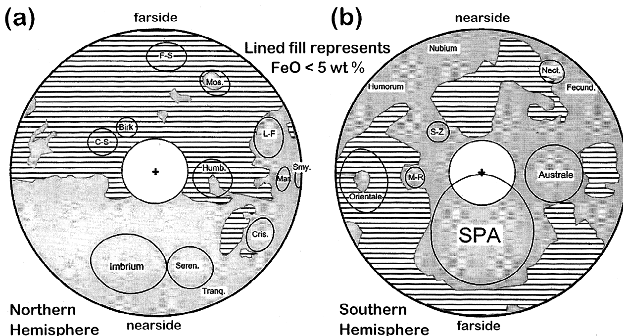
Figure 2. Polar projections of the lunar surface showing regions containing < 5 \text{ wt } \% \text{ FeO} as areas with lined fill: (a) northern hemisphere and (b) southern hemisphere. Approximate locations of major impact basins are outlined for reference. The large proportion of area in the northern hemisphere that has \text{FeO} < 5 \text{ wt } \% reflects the concentration there of the FHT highly anorthositic central region. In the northern hemisphere, regions that have > 5 \text{ wt } \% \text{ FeO} are associated mostly with the PKT. In the southern hemisphere, however, \text{FeO} -rich regions are also associated with SPA and in extensive regions associated with poorly defined, ancient basins such as Australe and possibly some extensive regions of cryptomare in the nearside southern hemisphere. Data are not shown for latitudes 75^\circ to the poles. \text{FeO} was derived from Clementine UVVIS [Lucey et al. , 1998a]. Abbreviations: C-S, Coulomb-Sartung; F-S, Freundlich-Sharanov; L-F, Lomonosov-Fleming; M-R, Mendel-Rydburg; S-Z, Schiller-Zucchius.
