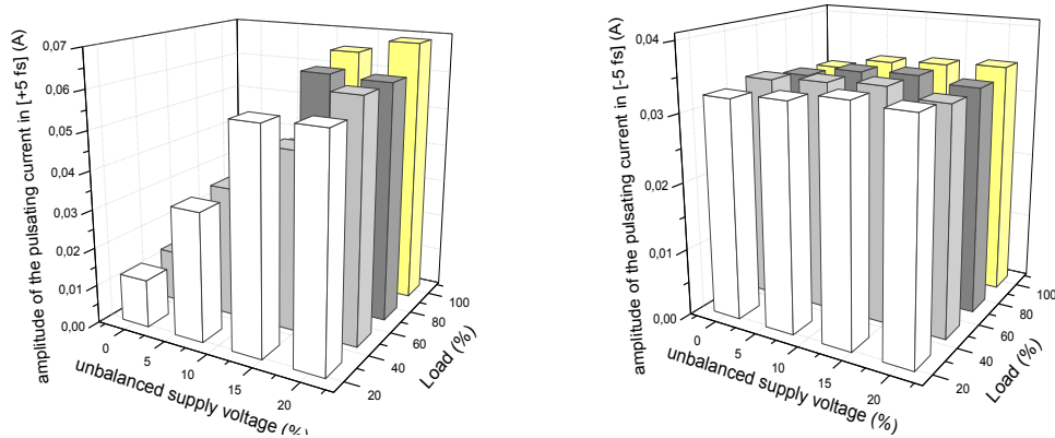
Figure 4. Analytical variation of the fifth positive (left) and the fifth negative (right) sequences harmonics according to the load percentage under different condition of unbalance supply voltage.
