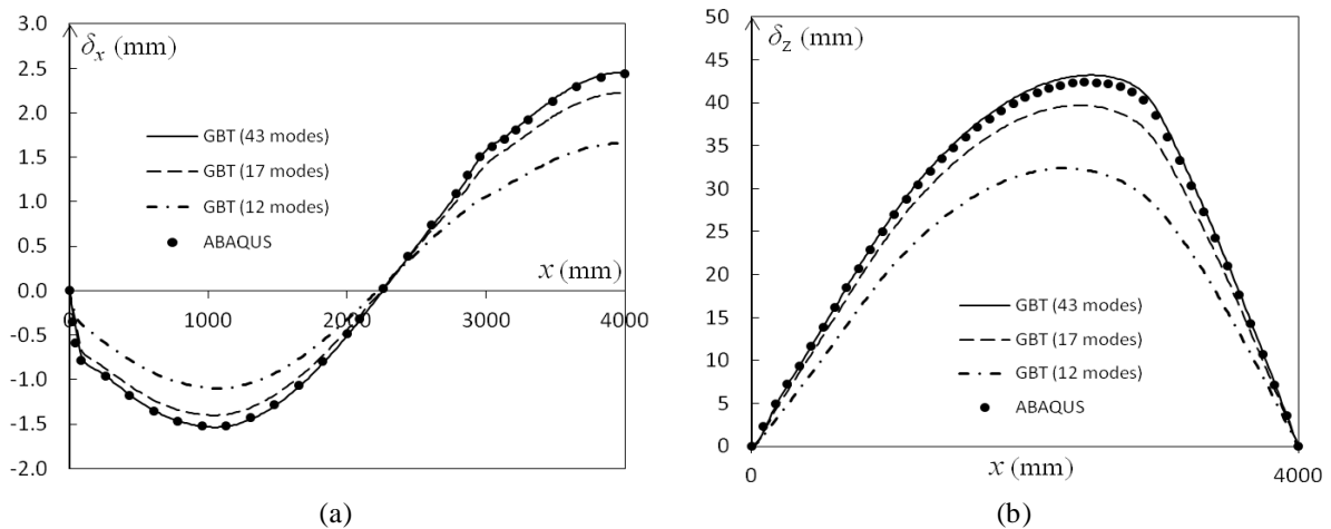
Figure 14: Top flange node (see Fig. 2(b)) (a) axial ( \delta_x ) and (b) transverse ( \delta_z ) displacement profiles at the P state ( \lambda_{\text{GBT}} = 104.1 ).
