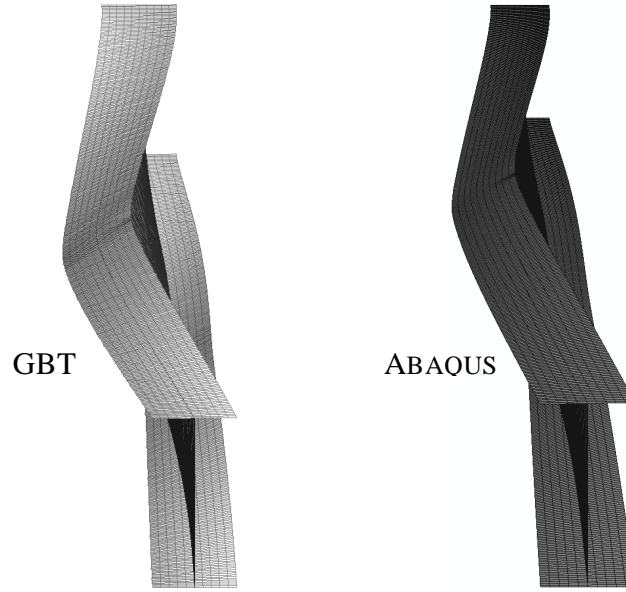
Figure 16: I-section beam collapse shape (AP equilibrium state).
