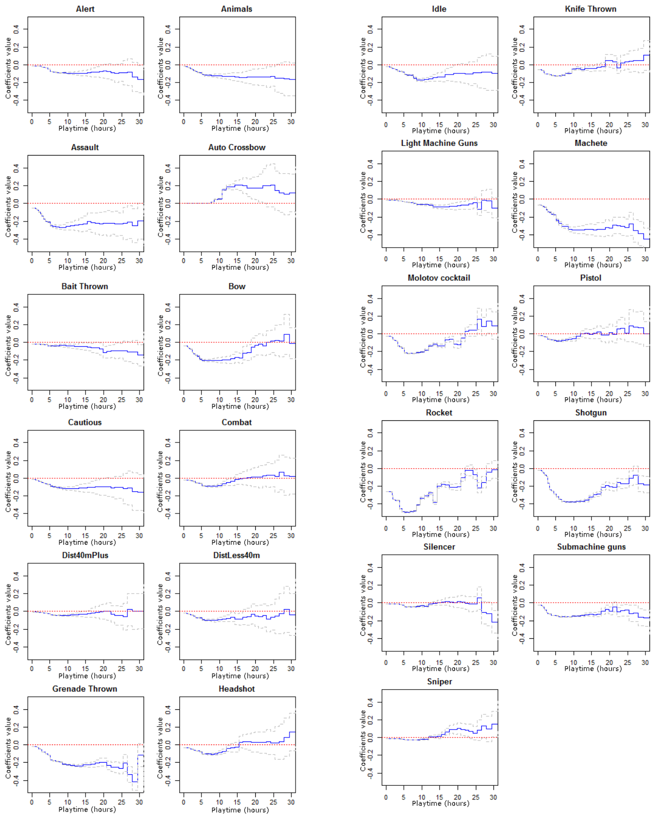
Fig. 6. Time varying coefficients (blue line) estimated on Far Cry 4 weapon usage dataset. Dashed grey line represent 95 % confidence intervals. Red dotted line at zero is the reference for null effect.
