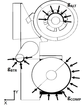
Figure 4: Load case
