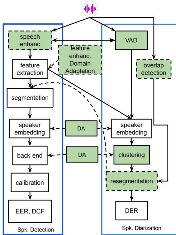
Fig. 1. Speaker detection pipeline. □ is the baseline system, □ are the new parts that are included in the pipeline, shaded-□ are the modules that were investigated.
