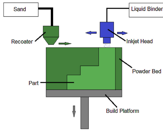
Fig. 2. A diagram of the binder jetting process, e.g. 3D sand mould printing. Acid mixed sand is spread by the recoater on the build platform and then the print head inkjets the binder according to each slice, cross-sectional area, of the part to be printed before it moves downwards and the process continues until the last slice is printed.
