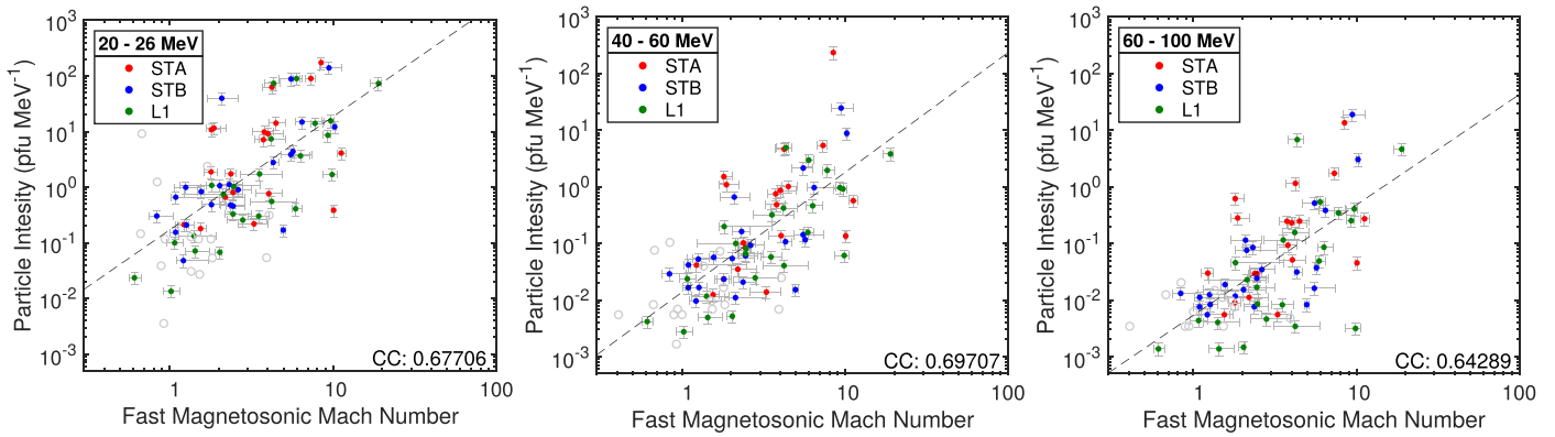
Figure 7. Comparisons between the SEP peak intensities and the fast magnetosonic Mach number ( M_{fm} ). See Figure 6 for more details.
