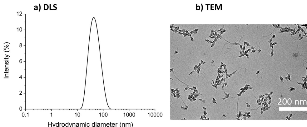
Fig. 2. AEP/HMP-stabilized apatite colloidal NP: a) particle size distribution (hydrodynamic diameters from DLS data) and b) TEM micrograph.
