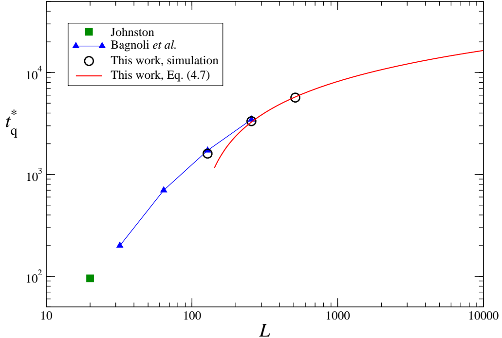
Figure 10: Time t_q^* for which P_L(t) has a maximum, as a function of L . The square data point for L = 20 is due to Johnston [25], the triangular ones for L = 32, 64, 128 , and 256 are due to Bagnoli et al. [21] and have been connected to guide the eye, and the circular ones, for L = 128, 256 , and 512 , were obtained in this work. The red line is the large L expansion [equation (4.7)] of our heuristic theory.
