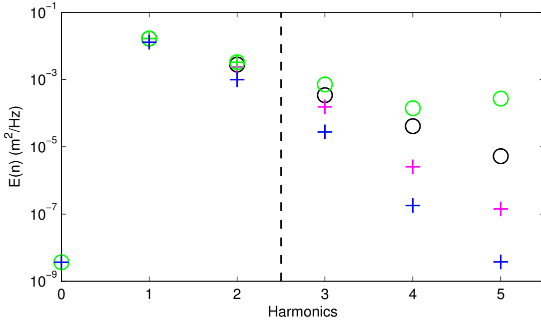
Figure 3: Surface elevation energy density spectra E(n) of a periodic weakly nonlinear wave, \epsilon = 0.15 , \mu = 0.25 , \delta_m = 0 . Full Euler solution (black circle); hydrostatic reconstruction: \zeta_H^{\delta_m} (blue crosses); linear formula in space: \zeta_{L,space} (magenta crosses); TFM - no cutoff: \zeta_{L,NC} (green crosses); TFM - sharp cutoff: \zeta_{L,Sh} (green circles); see the associated equations in Tab. 1. The cutoff harmonic index is indicated by the vertical black dotted line.
