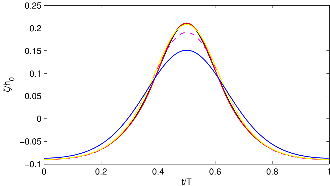
Figure 4: Surface elevation of a periodic weakly nonlinear wave, \epsilon = 0.15 , \mu = 0.25 , \delta_m = 0 . Full Euler solution (black line); hydrostatic reconstruction: \zeta_H^{\delta m} (blue line); linear formula in space: \zeta_{L,space} (magenta dashed line); fully-dispersive nonlinear reconstruction in space: \zeta_{NL,space} (red line); heuristic reconstruction in space: \zeta_{HE,space} (yellow line); see the associated equations in Tab. 1 and 2.
