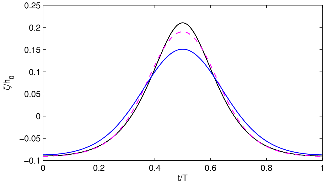
Figure 2: Surface elevation of a periodic weakly nonlinear wave, \epsilon = 0.15 , \mu = 0.25 , \delta_m = 0 . Full Euler solution (black line); hydrostatic reconstruction: \zeta_H^{\delta_m} (blue line); linear formula in space: \zeta_{L,\text{space}} (magenta dashed line); see the associated equations in Tab. 1.
