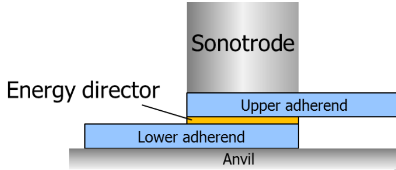
Figure 7: Principle of ultrasonic welding of thermoplastic composites using a flat energy director.
