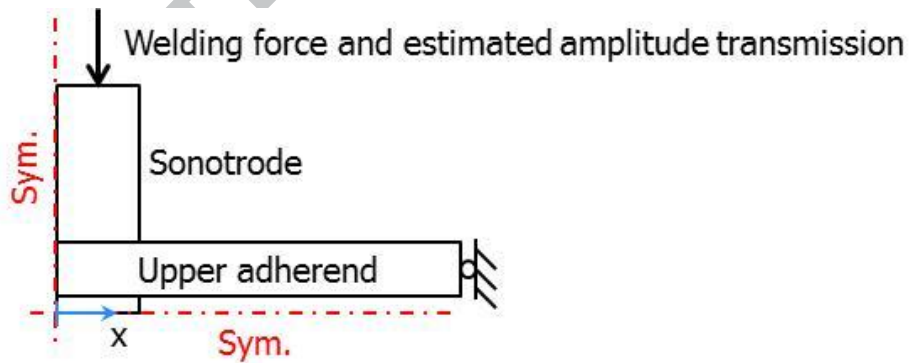
Figure 10: Boundary conditions of 2D model to predict the power dissipated during the ultrasonic welding process. A quarter model was used based on the symmetry (Sym.) of the system.
