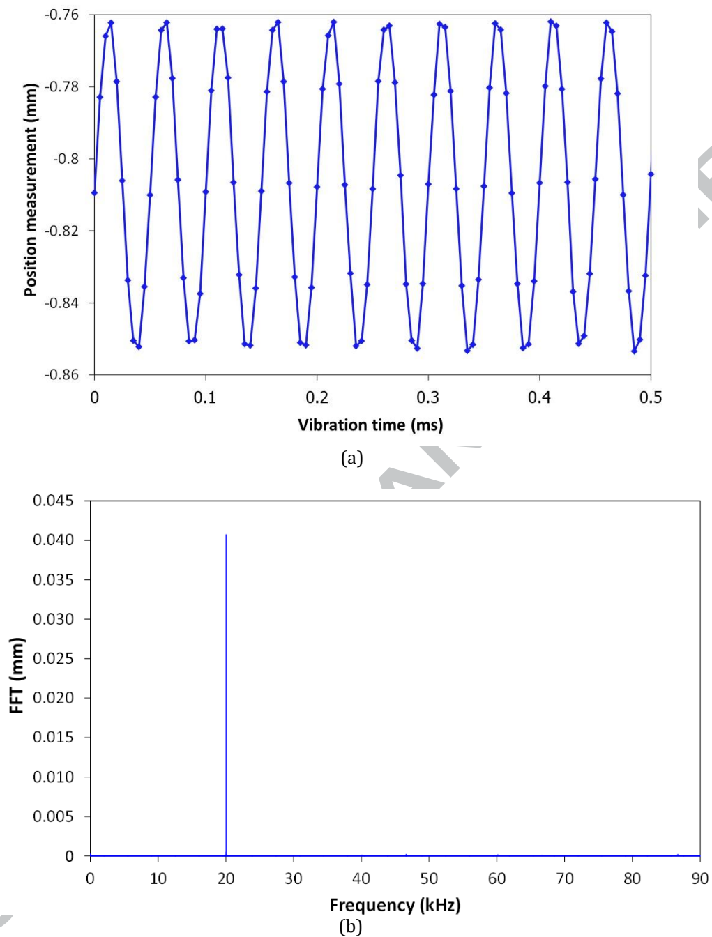
Figure 12: (a) Representative example of the measured sonotrode displacement using a laser sensor at position 1 (as shown in Figure 11) with a nominal amplitude of 45.4 \mu\text{m} . (b) Corresponding Fast Fourier Transformation (FFT).
