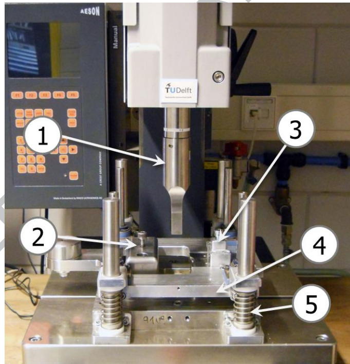
Figure 8: Ultrasonic welding setup used in this work. 1: Sonotrode, 2: clamp for lower adherend, 3: clamp for upper adherend, 4: moving platform, and 5: springs supporting the moving platform.
