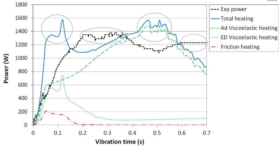
Figure 13: Comparison between experimental (Exp power) and simulated (Total heating) power curves for a representative welding case (1500 N welding force and 36.3 \mu\text{m} nominal amplitude) using average amplitude from Figure 12. Viscoelastic heating from adherends: Ad Viscoelastic heating, viscoelastic heating from energy director: ED Viscoelastic heating, frictional heating: Friction heating. The circled areas represent two characteristic power peaks for both simulated and experimental curves.
