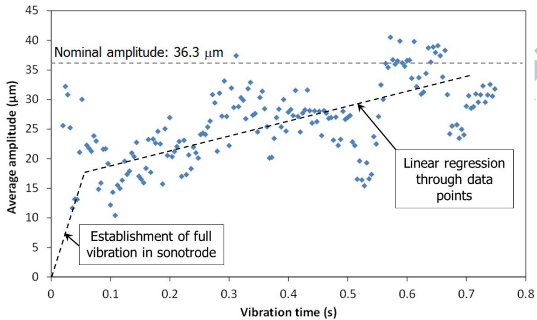
Figure 12: Evolution of the estimated amplitude transmitted to the upper adherend (1500 N welding force and 36.3 \mu\text{m} nominal amplitude). Values were calculated at 0.004 s time intervals over the duration of the process, an affine function was fitted through the data points and a linear increase of the amplitude was proposed during the period needed for full amplitude to be established in the sonotrode.
