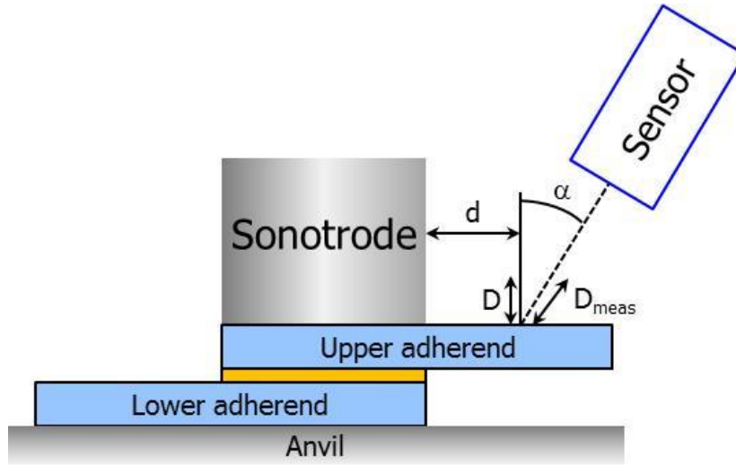
Figure 9: Determination of amplitude transmission via displacement measurement of the upper adherend during ultrasonic welding using a tilted sensor. Measured displacement: D_{meas} , real displacement: D , sensor tilt angle: \alpha , and distance between sonotrode and laser: d . Dimensions are not to scale.
