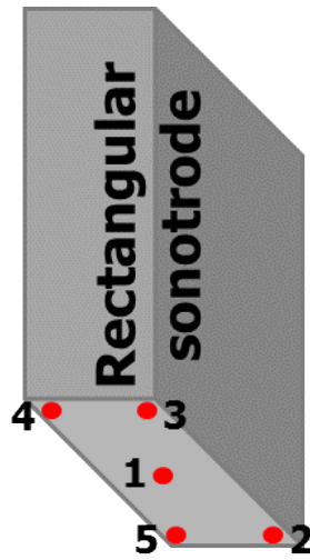
Figure 11: Displacement sensor positions on the bottom surface of the sonotrode for calibration measurements.
