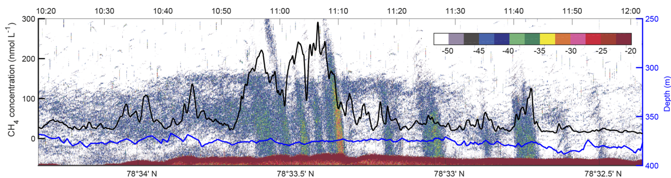
Figure 5. Towed MILS data overlaying echo-sounder data. The black line shows the \text{CH}_4 concentration along line 3 (see Fig. 1 for location) at \sim 15 m from the seafloor. The blue line indicates the depth of the probe. The echogram, displaying target strength values (colour bar shows intensity – dB) from the 38 kHz channel of the EK60, is shown in the background.
