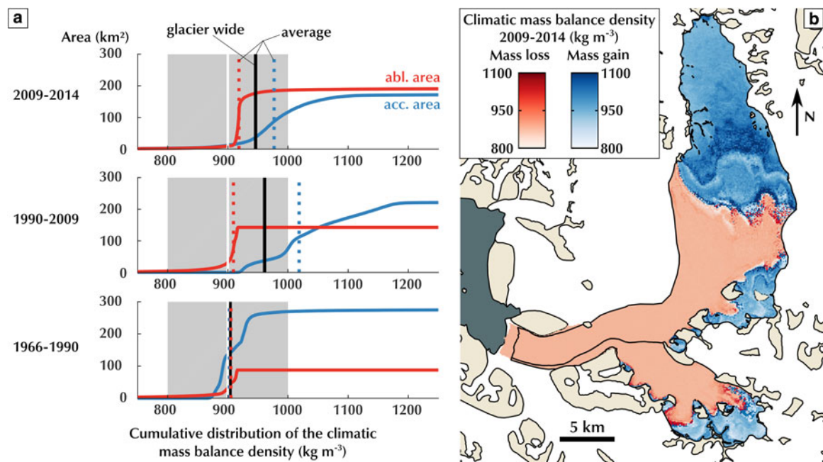
Fig. 7. Volume change to mass change conversion factor in the climatic mass-balance model. (a) Cumulative distribution of the density of the climatic mass loss (red line) and gain (blue line). Vertical line shows the average density of the climatic mass changes for the ablation area (dotted red), accumulation area (dotted blue) and the entire glacier (full black). Vertical white line shows the conversion factor used for calculation of the geodetic mass balance with error range (grey box). (b) Map of the density of the climatic mass change over KRB between 2009 and 2014. Blue shades show mass gain area, red shades show mass loss area.
