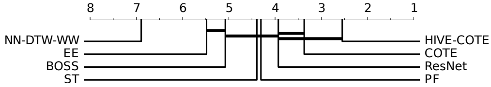
Fig. 8: Critical difference diagram showing pairwise statistical difference comparison of state-of-the-art classifiers on the univariate UCR/UEA time series classification archive.
