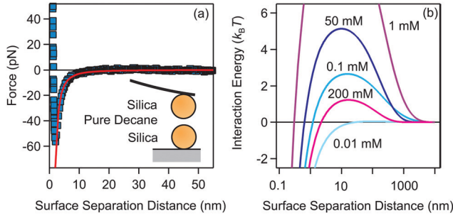
Fig. 3 (a) van der Waals interaction measured between two 4\ \mu\text{m} silica spheres measured in pure decane. The line represents the fit to non-retarded van der Waals expression with the Hamaker constant H = (1.8 \pm 0.2) \times 10^{-21} J. (b) DLVO interaction energies for 200 nm silica particles in decane for different AOT concentrations, calculated with eqn (8). The measured Hamaker constant was used to calculate the van der Waals interaction, while electrokinetic potential and conductivity measurements were used to calculate the double-layer interaction.
