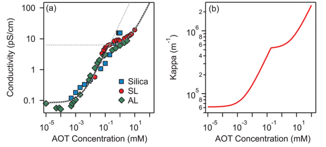
Fig. 1 (a) Conductivity and (b) inverse Debye length \kappa versus concentration of AOT in decane solutions containing silica, SL, and AL particles. The dashed lines in (a) are linear fits for conductivity below and above the CMC; the full line shows the interpolation fit. Note that the conductivity values obtained in solutions without particles are the same as those in particle suspensions within experimental error. The contribution of colloids to conductivity is therefore negligible.
