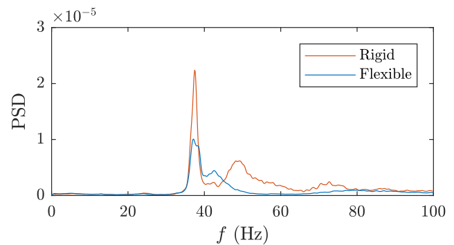
Figure 3. Narrowband X force power spectral density (PSD) for the rigid and flexible hydrofoils at \sigma = 0.8 , Re_c = 0.7 \times 10^6 and \alpha = 6^\circ .
