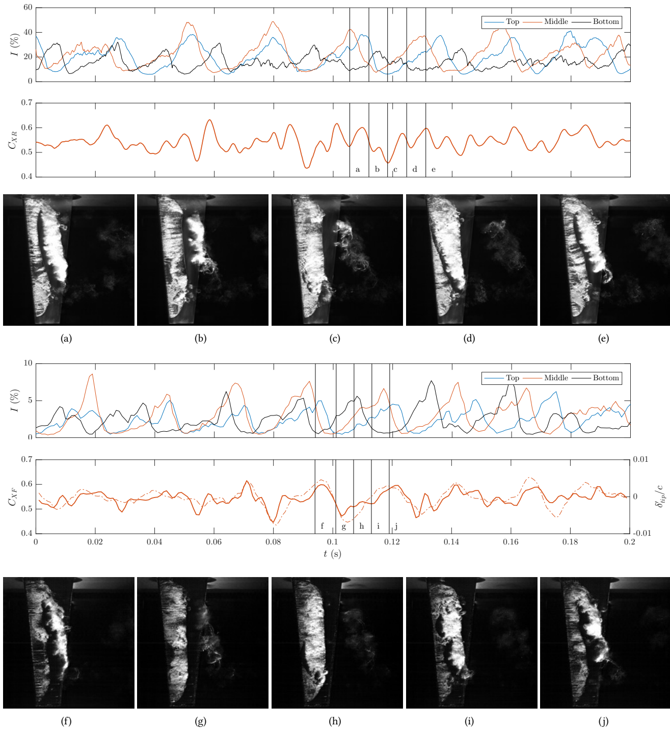
Figure 4. Sample time series of normal force coefficient with selected images from high-speed imaging for the rigid (top) and flexible hydrofoil (bottom). Simultaneous normalized unsteady tip bending displacement (dot-dashed line) is also presented for the flexible hydrofoil. The 3 curves of pixel intensity are taken at 75% of the chord for span-wise locations of 0.24s, 0.47s and 0.77s from the root. Data was taken at \sigma = 0.8 , Re_c = 0.7 \times 10^6 and \alpha = 6^\circ .
