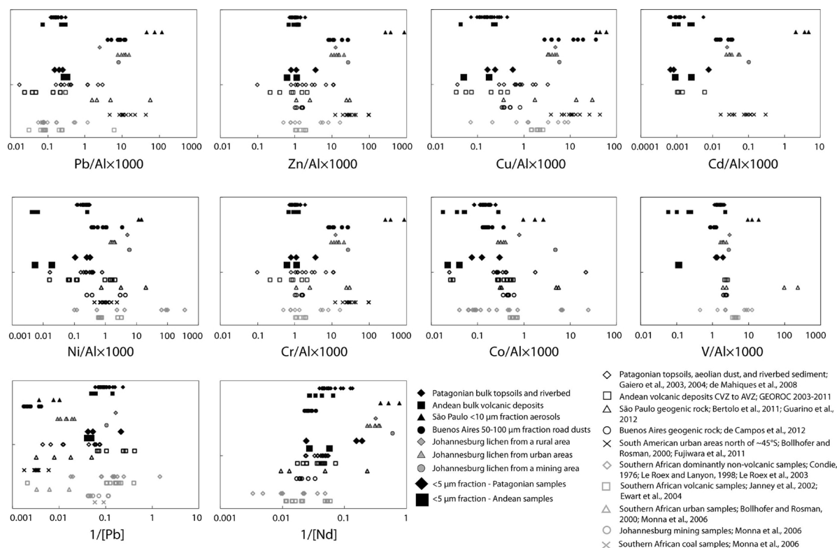
Fig. 2. Selected trace element/Al ratios, and 1/[Pb], 1/[Nd] data for samples from this study (filled symbols) and the literature (open symbols). All measurement uncertainties are smaller than the size of the symbols.
