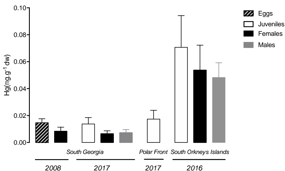
juveniles were found at this location Figure 2- Total mercury concentrations ( \mu\text{g g}^{-1} \text{dw} ) in Antarctic Krill ( Euphausia superba ) collected around South Georgia and at the Antarctic Polar Front in the austral summer of 2016/17, and around the South Orkney Islands during the austral summer of 2015/16. Bars show the mean. Error bar is 1 standard deviation.
