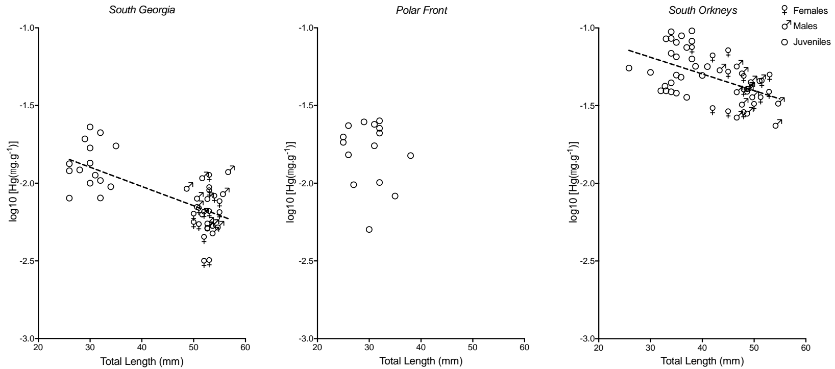
Figure 3 – Total mercury concentration ( \mu\text{g g}^{-1} dw) on a log10 scale versus total length (mm) for individual Antarctic krill ( Euphausia superba ) by maturity stage and sex respectively. Data are shown separately for krill collected around South Georgia ( Y = -0.0124 \cdot X - 1.525 , R^2 = 0.46 , F_{1, 43} = 36.41 , p < 0.001 ), the Antarctic Polar Front (both in the austral summer of 2016/17) and the South Orkney Islands ( Y = -0.01072 \cdot X - 0.8675 , R^2 = 0.2746 , F_{1, 52} = 19.69 , p < 0.001 ; summer of 2015/16).
