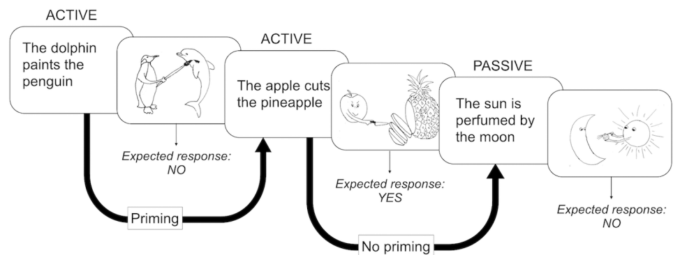
Fig 2. Structure of the homogenous and heterogeneous blocks used in the experiment. The top panel illustrates the structure of a homogeneous block, using the example of a passive block. The bottom panel illustrates the structure of a heterogeneous block, in which both active and passive sentences are presented. Thick arrows indicate whether or not priming is expected between two consecutive sentences. Expected responses on the sentence-picture pairs are also indicated.
