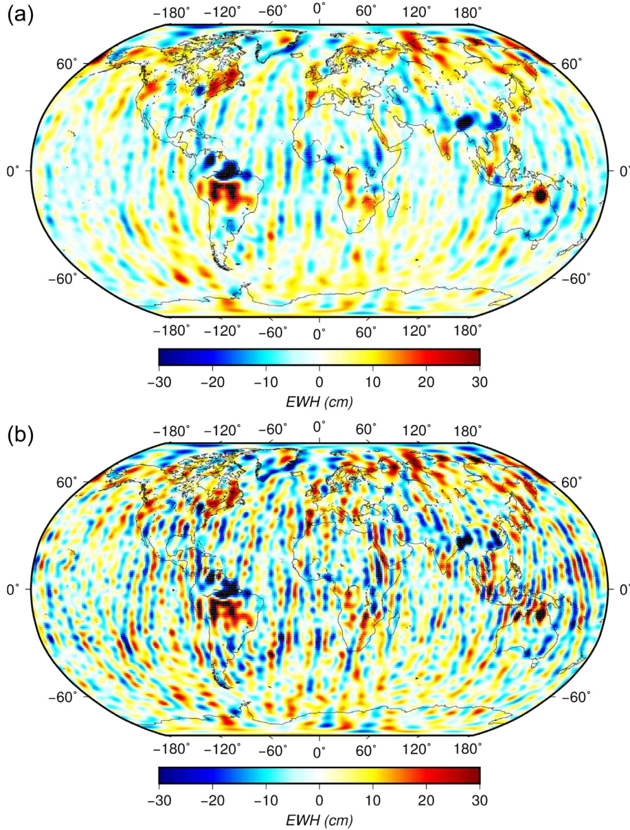
Figure 1. Surface mass density anomaly solutions for January 2006, relative to July 2005, expressed in equivalent water height (EWH, in cm): (a) mean of CSR, GFZ and JPL solutions derived from GRACE and filtered using the decorrelation filter DDK5 and (b) mean of CSR, GFZ, GRAZ, GRGS and JPL solutions filtered with DDK7.
