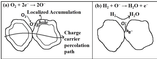
Fig. 3. Schematic of the proposed sensing mechanism- (a) during stabilization of the sensor material (oxygen adsorption); (b) during sensing of the test gas (e.g. hydrogen).
