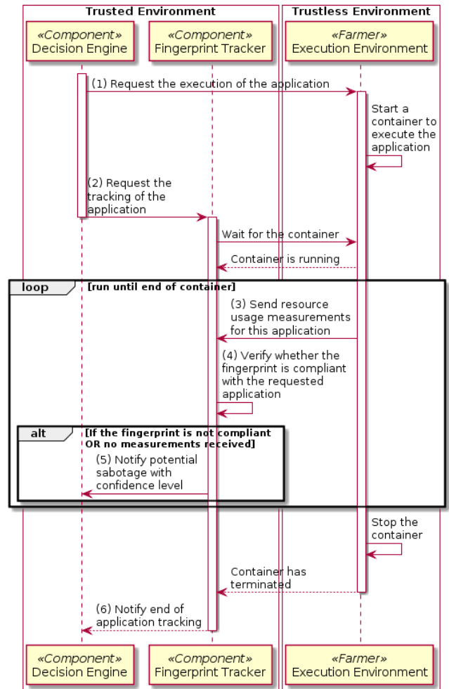
Figure 3. Sequence diagram of the interaction between the trusted environment and the trustless environment
