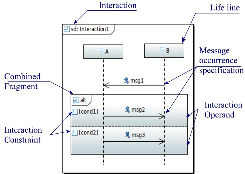
Figure 3: Sequence diagram elements
