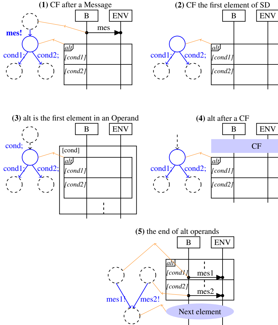
Figure 7: Alt transformations
