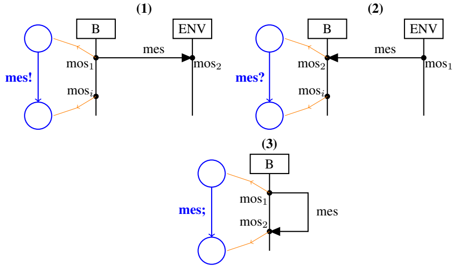
Figure 6: Message transformation
