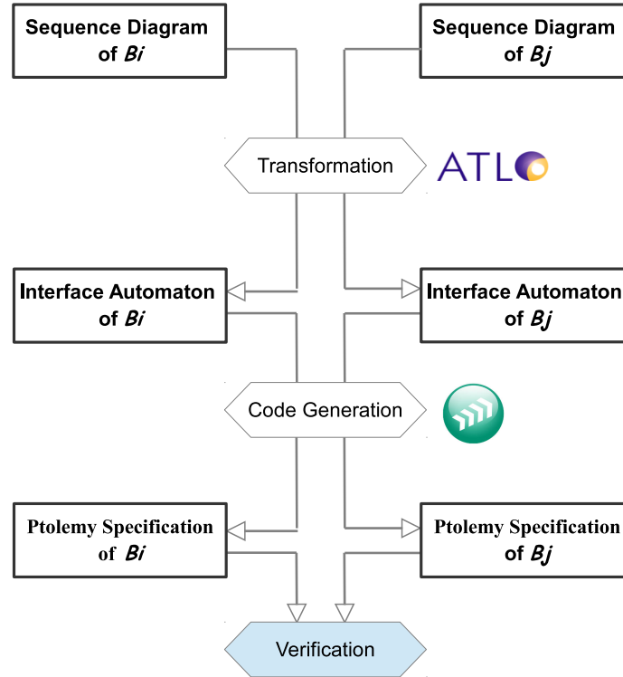
Figure 1: Our Methodology
