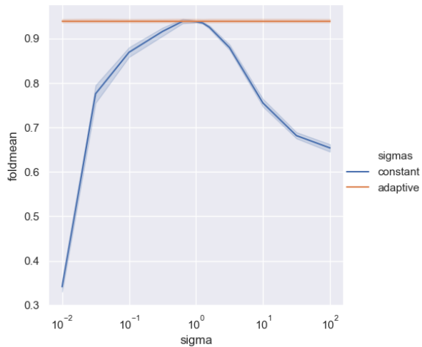
Figure 3: Classification accuracy and deviations for Orbit5K as \sigma_1, \dots, \sigma_b = \sigma is varied (in blue), compared to the adaptive strategy of Equation (2) (orange).
