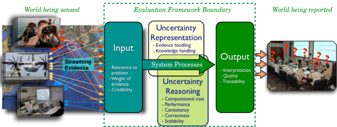
Fig. 2. URREF Boundary. This figure depicts the world being sensed on the left, the role of uncertainty representation and reasoning within a fusion system in the center, and the world being perceived on the right. The evaluation framework boundary encompasses the fusion system input, uncertainty representation, uncertainty reasoning and the fusion system output. Everything inside the evaluation framework boundary is known as the Uncertainty Representation and Reasoning Framework (URREF). The uncertainty representation and uncertainty reasoning are the primary subjects of evaluation, whereas the input and output are secondary subjects of evaluation.
