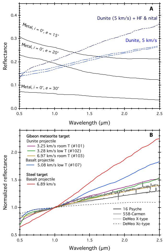
Fig. 5. VIS-NIR spectra of the produced craters compared to observation of probable metal-rich asteroids. (A) VIS-NIR spectra of the craters produced with a dunite projectile, run n5 at 4.91 km/s. The black spectra show the spectral signature of the metal outside of the crater and its dependency on observation geometry (same incidence angle, 0^\circ ; three different emergence angles, 15^\circ , 20^\circ , and 30^\circ ). The light blue spectra were measured inside the crater (incidence, 0^\circ ; emergence, 20^\circ ). The dark blue spectra were measured after treating the sample with HF-nital, removing the material coating the crater floor (i.e., glassy dunite). The removal of this material induces an increase of the overall reflectance level. (B) Normalized reflectance spectra of the craters produced in this study compared to observation of probable metal-rich asteroid (14) as well as metal-related spectral end-members (36). The obtained craters show variations of spectral slopes, including slope values similar to ground-based observation of probable metal-rich asteroids.
