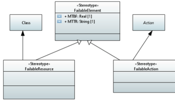
Figure 6 : UML Profile for loading Weather FMU
