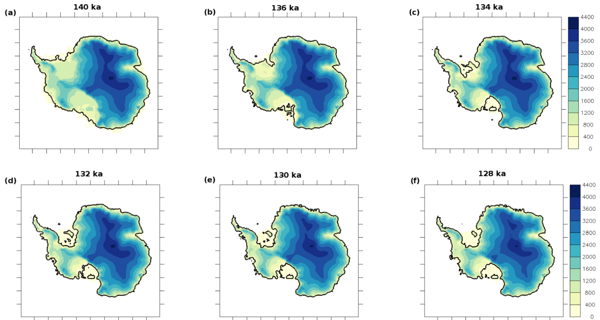
Figure 6. Antarctic ice-sheet elevation at (a) 140 ka, (b) 136 ka, (c) 134 ka, (d) 132 ka, (e) 130 ka and (f) 128 ka as simulated by the GSM (e.g. Briggs et al., 2014). Grounding lines are in black.
