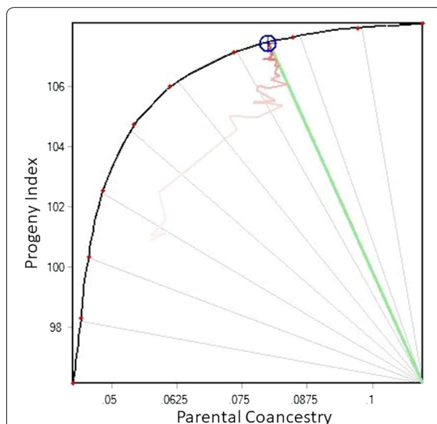
Fig. 1 An example frontier response surface involving progeny index and parental coancestry. Reproduced from [39] with permission
