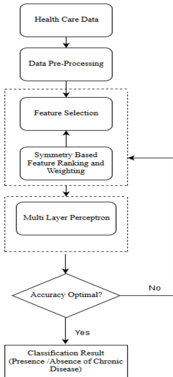
Fig. 1.Proposed Architecture Diagram
