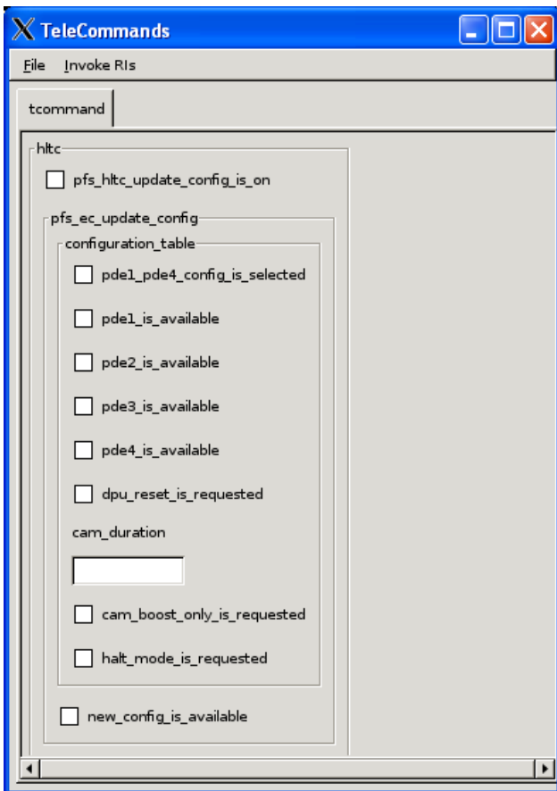
Figure 8: Auto-generated GUI
