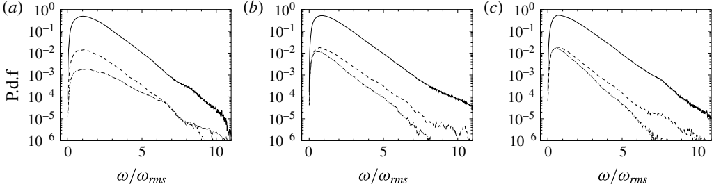
FIGURE 20. Total and conditional p.d.f. of the normalized vorticity magnitude: (a) air; (b) PP11-IC1; (c) PP11-IC2; —, [-\infty, +\infty] ; ---, [-\infty, -2] ; - · · -, [2, \infty] .
