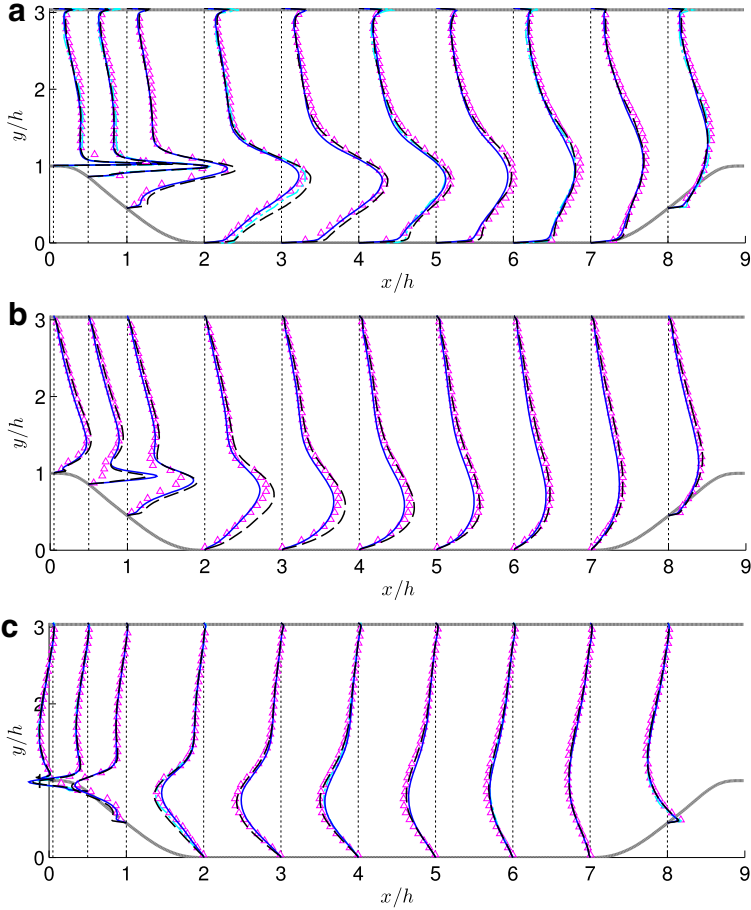
Fig. 21 Periodic hill flow at Re = 19000 : (—) RT 256 \times 128 \times 128 ; (— —) RT 512 \times 256 \times 256 ; ( \Delta\Delta ) experiments Rapp & Manhart [24]; (— · — ·) DG LES of de la Llave Plata et al. [75]. Turbulent intensities \langle u'u' \rangle a , \langle v'v' \rangle b , \langle u'v' \rangle c
