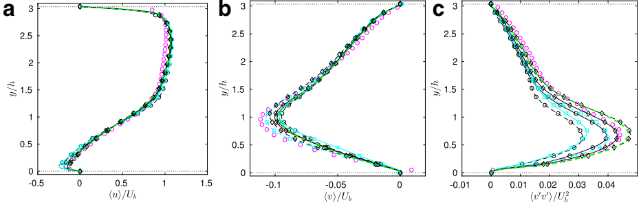
Fig. 18 Influence of subgrid-scale models at Re = 10595 : SM C_S=0.18 ( \blacktriangle ), SM C_S=0.1 ( \circ ), DSM C_d ( \square ), DSM C_d/2 ( \square ), MSM-ls ( \blacktriangle ), MSM-ss ( \circ ) and RT ( \blacksquare ). \circ PIV measurements of Rapp & Manhart [10, 24]. Profiles of \langle u \rangle a ; \langle v \rangle b and \langle v'v' \rangle c at x/h = 3
