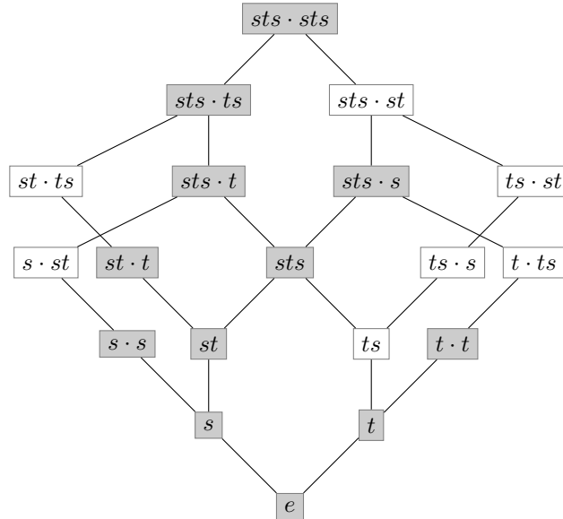
Fig. 1: \text{Weak}^{(2)}(A_2) . The elements marked in gray are the st -sortable elements.
