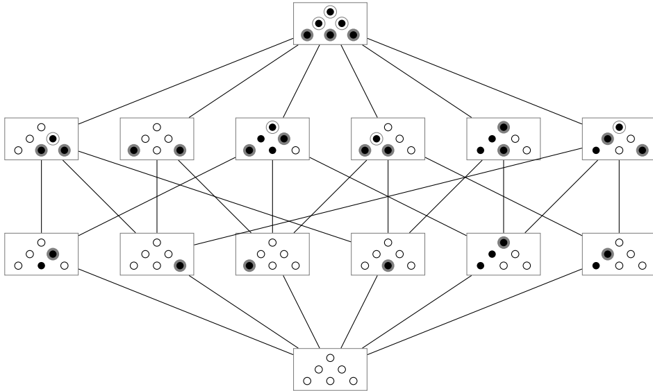
Fig. 5: \text{Shard}(A_3) restricted to \text{Sort}(A_3, s_1 s_2 s_3) . Sortable elements are given by their inversion sets in the positive roots. Covered reflections are circled in grey, and further inversions in the parabolic subgroup generated by the covered reflections are circled in white.
