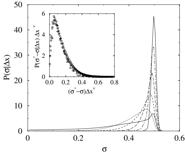
FIG. 4. Distribution of depinning stress (bold line) and contributions conditioned by the distances (2, 4, 8, 16, 32) between consecutive active sites. The tail of the distribution corresponds to very short jumps and is very sensitive to the details of the random threshold distribution. The contributions obtained for increasing distances between consecutive active sites present the same trend: the larger the jump, the closer the mean force to the threshold and the narrower the distribution. After rescaling (inset) these distributions collapse onto a single master curve.
