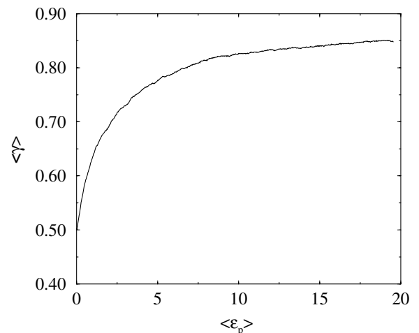
FIG. 1. Evolution of the mean yield threshold \langle \gamma \rangle versus the plastic strain \langle \varepsilon_p \rangle during the transient regime of a first loading process. The increase of \langle \gamma \rangle can be interpreted as a hardening effect.
