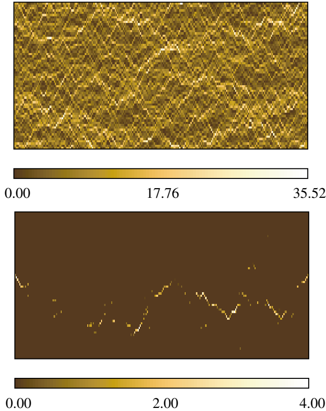
FIG. 2 (color online). Map of the relative displacement field obtained on a system 128 \times 64 after 800 000 time steps (top). The diffuse localization corresponds to the successive development of anisotropic structures elongated in the longitudinal direction. Focusing on a finite time window (450 time steps, bottom) allows one to reveal an individual structure.
