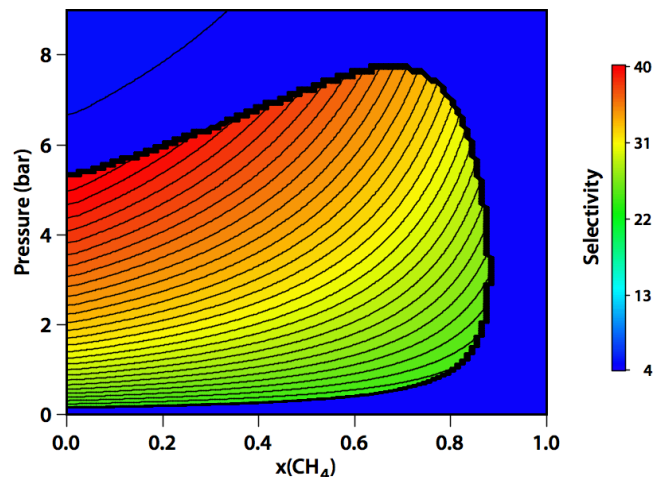
Figure 7. Diagram indicating the CO_2 selectivity upon adsorption of a CO_2/CH_4 mixture in MIL-53 (Al) at 300 K, as predicted by the OFAST method, as a function of mixture composition ( x axis) and total gas pressure ( y axis). The inner, high-selectivity island correspond to the np phase, delimited from the lower-selectivity lp phase by a wide black line. Reprinted with permission from ref. 114.
