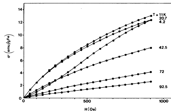
FIG. 10. In an Fe_{0.33}Sn_{0.67} amorphous alloy the isothermal magnetization curves are not monotonous functions of T in their lowest-field part.
