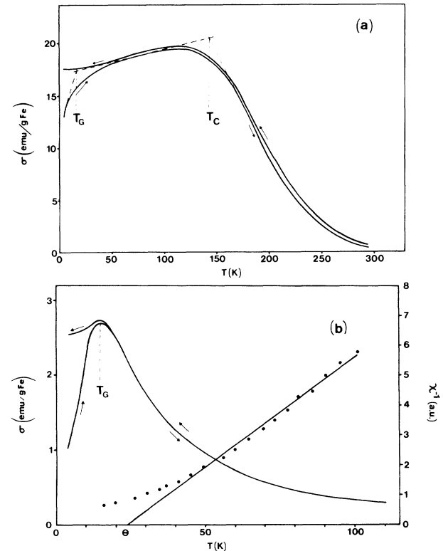
FIG. 1. Typical isofield magnetic curves obtained from various \text{Fe}_x\text{Sn}_{1-x} amorphous alloys where (a) x=0.43 and (b) x=0.33 , with an applied external field H=100 Oe. Arrows indicate that \sigma(T) is measured with increasing or decreasing temperatures. In (b) the temperature dependence of the reciprocal susceptibility is also shown. (Hysteresis observed up to 300 K might be an experimental artifact due to difference in heat-transfer velocity when cooling and warming samples.)
