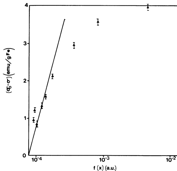
FIG. 17. Typical unsuccessful test (even within error bars) of a model of macroscopic magnetic inhomogeneity. Plot of \sigma - \sigma' vs f(x) [ f(x) defined in text] for a \text{Fe}_{0.37}\text{Sn}_{0.63} amorphous alloy.
